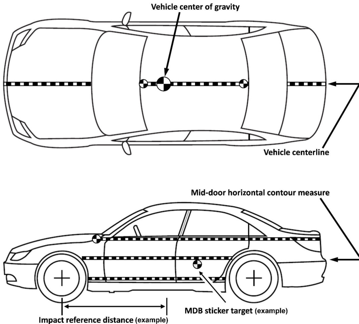
Figure 4 Exterior surface marking
