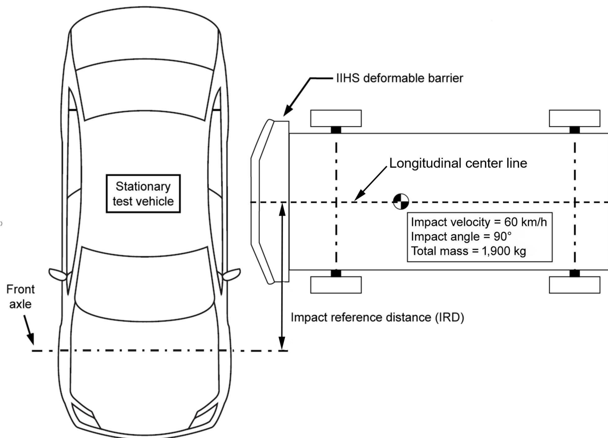
Figure 1 Moving deformable barrier alignment with test vehicle
