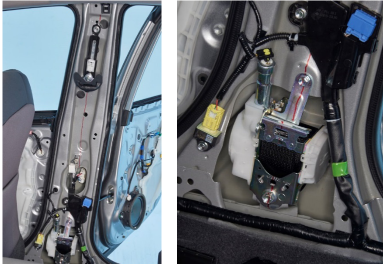
Figure 8 Example of interior B-Pillar and crash tensioner profile measure — Precrash
