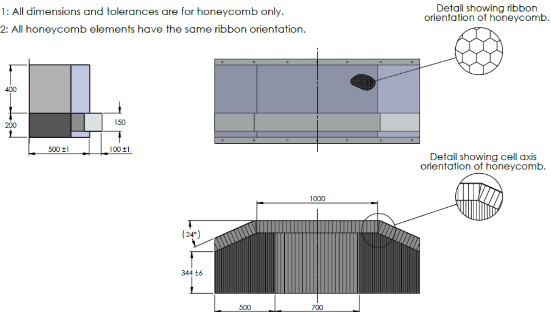
Figure 3 IIHS deformable barrier element (all dimensions in millimeters)
