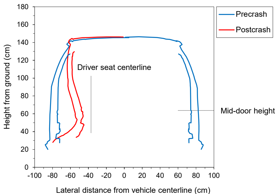
Figure 7 Example B-Pillar vertical profiles
