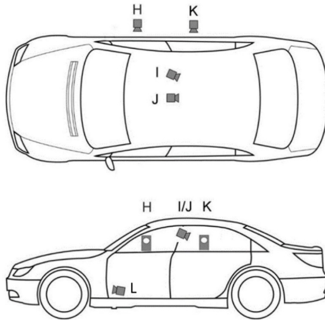
Figure 6B Onboard high-speed camera positions
