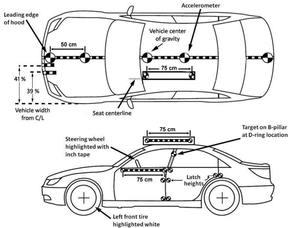
Figure 4 Exterior surface marking
